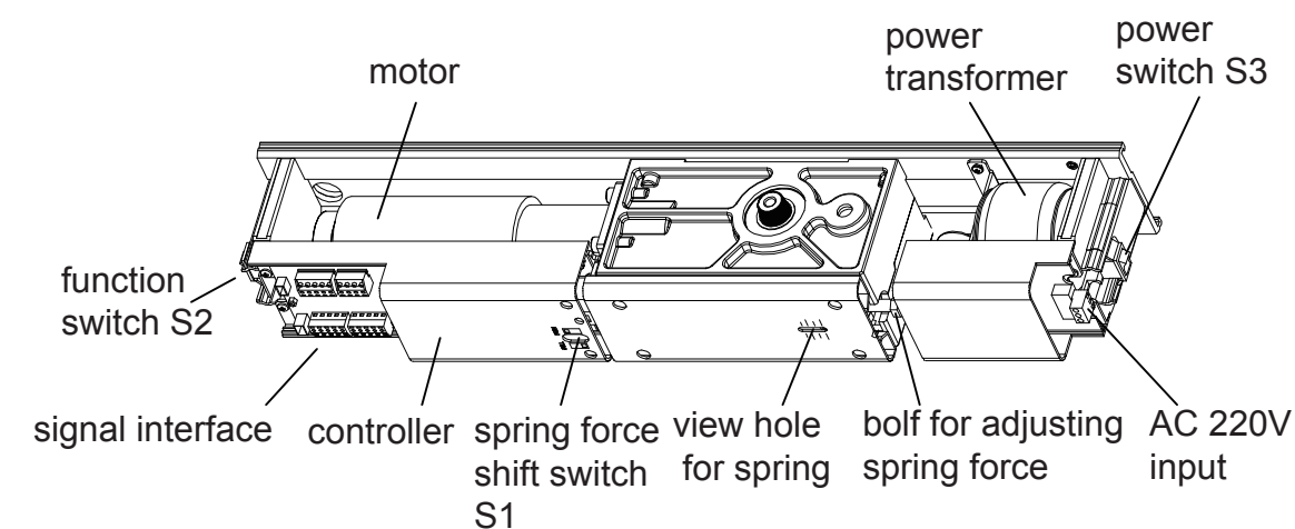
Drive device
